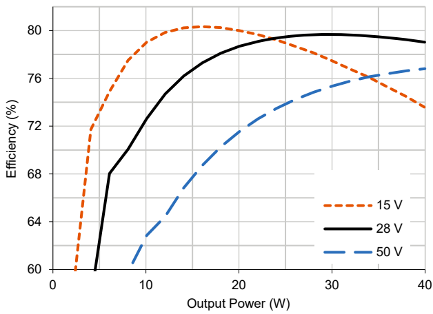
4.3.1 SVLTR2812D Efficiency (Typical, 25 °C)
