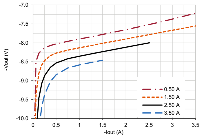
4.3.2 SVLTR2812D Cross-Regulation (Typical, 25 °C)
