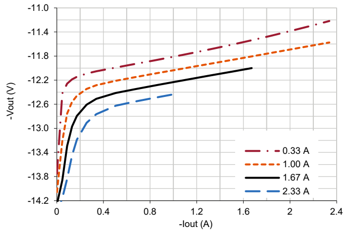
4.3.2 SVLTR2812D Cross-Regulation (Typical, 25 °C)
