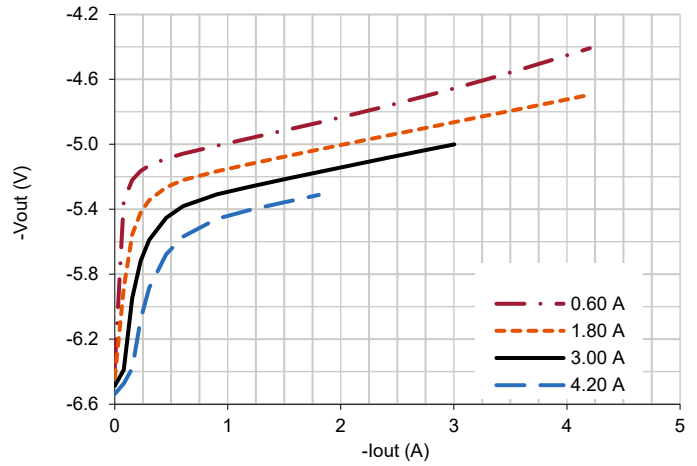
4.1.2 SVLTR2805D Cross-Regulation (Typical, 25 °C)
