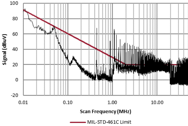
4.1.1 Two VXR250-2800S without EMI Filter
