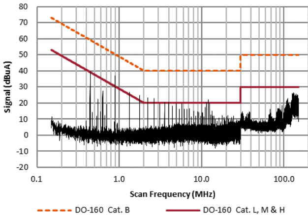
4.1.5 Two VXR250-2800S without EMI Filter
