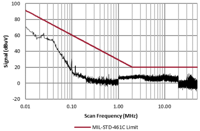
4.1.2 Two VXR250-2800S with EMI Filter
