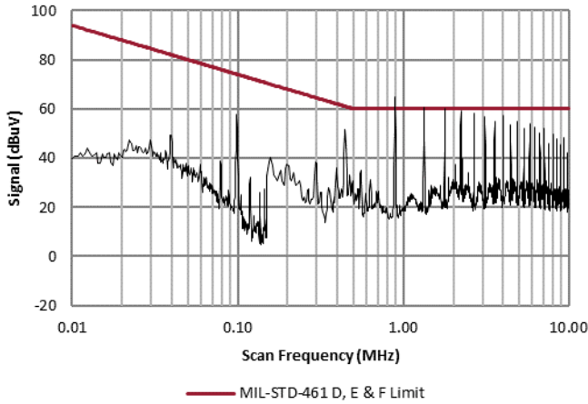
4.1.3 Two VXR250-2800S without EMI Filter
