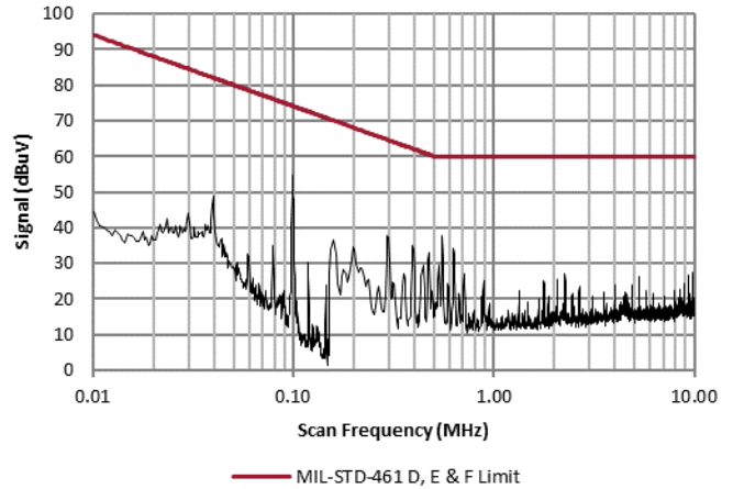
4.1.4 Two VXR250-2800S with EMI Filter
