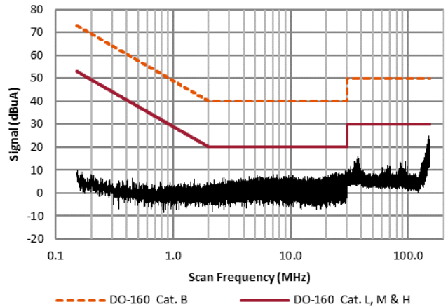
4.1.6 Two VXR250-2800S with EMI Filter
