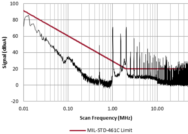
4.1.1 Two VXR100-2800S without EMI Filter
