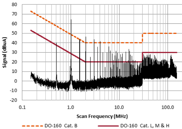
4.1.5 Two VXR100-2800S without EMI Filter
