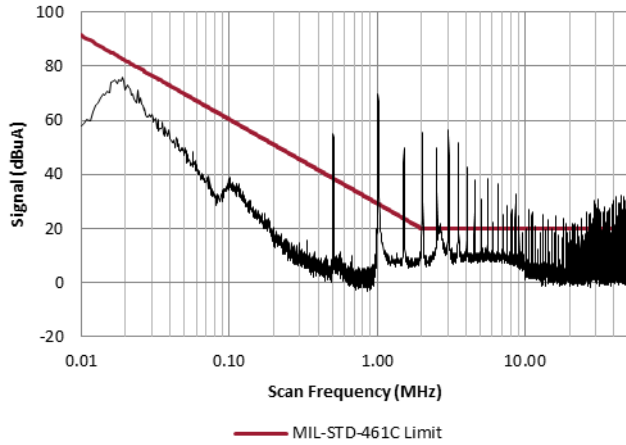
4.1.1 VXR100-2800S without EMI Filter
