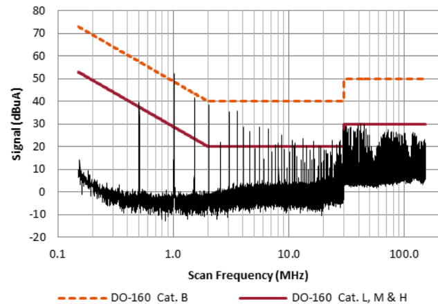
4.1.5 VXR100-2800S without EMI Filter
