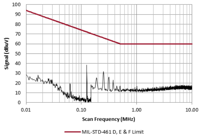
4.1.4 VXR100-2800S with EMI Filter
