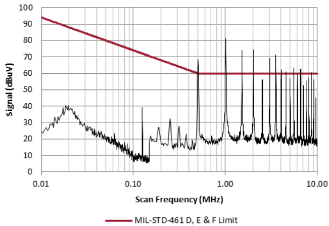
4.1.3 VXR100-2800S without EMI Filter
