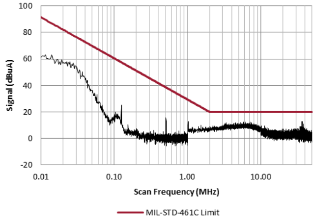
4.1.2 VXR100-2800S with EMI Filter
