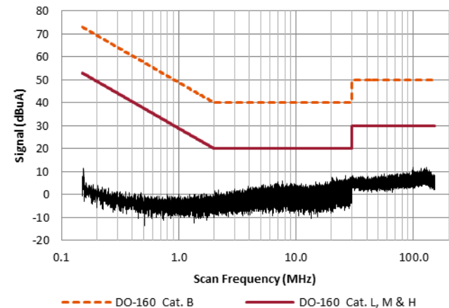
4.1.6 VXR100-2800S with EMI Filter
