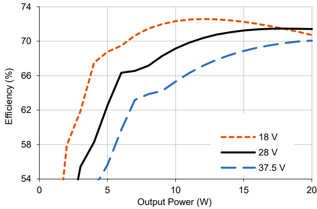
4.1.1 SVRTR283R3S Efficiency (Typical, 25 °C)
