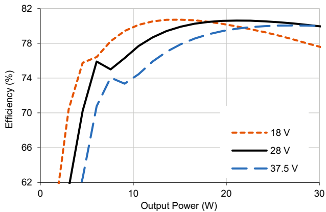
4.1.5 SVRTR2815S Efficiency (Typical, 25 °C)
