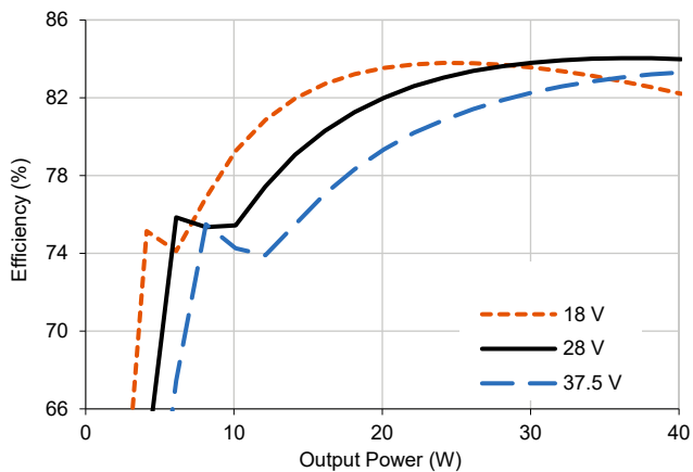
4.1.5 SVRTR2815S Efficiency (Typical, 25 °C)
