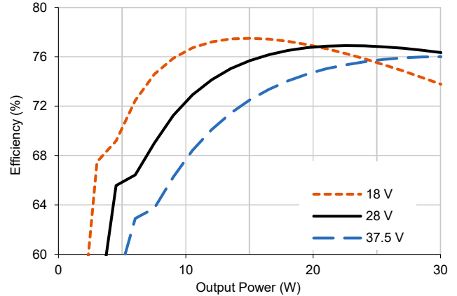
4.1.2 SVRTR2805S Efficiency (Typical, 25 °C)
