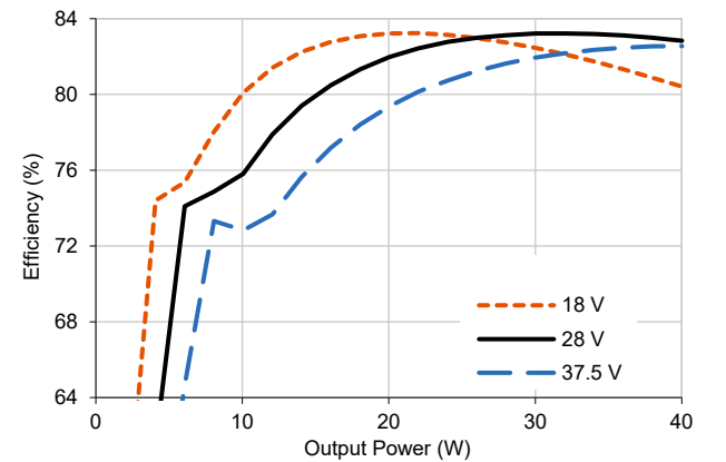
4.1.4 SVRTR2812S Efficiency (Typical, 25 °C)
