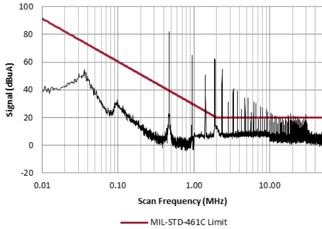
4.1.1 Two VSC15-2800S without VSCF3-28 EMI Filter
