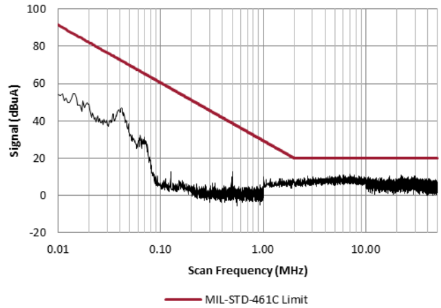
4.1.2 Three VSC30-2800S with VSCF10-28 EMI Filter
