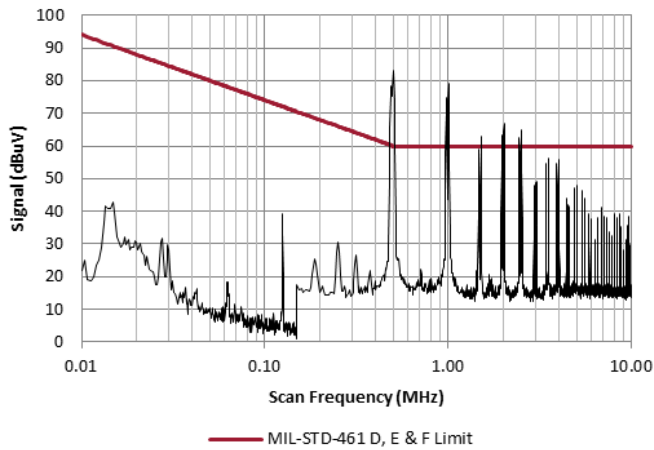
4.1.3 Three VSC30-2800S without VSCF10-28 EMI Filter
