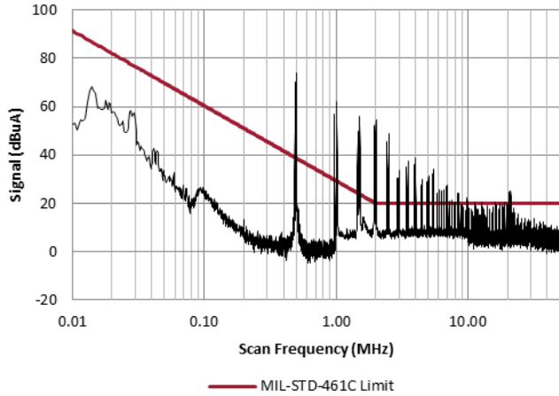
4.1.1 Three VSC30-2800S without VSCF10-28 EMI Filter
