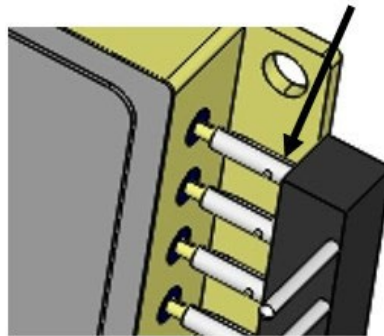
Figure 7: Up Lead and Down Lead solder pour area.
