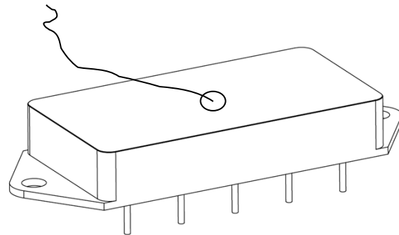
In-correct Thermocouple Placement
