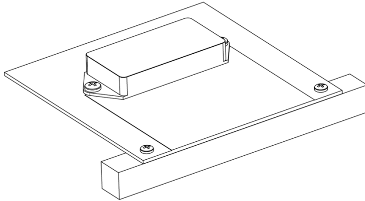
Figure 3. – Thermal copper plane used to carry heat from the converter to a chassis or heatsink.
