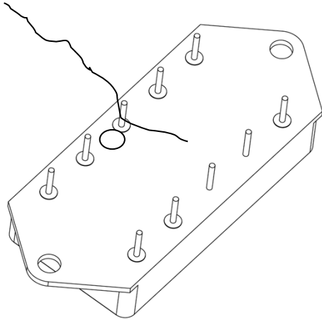
Correct Thermocouple Placement
