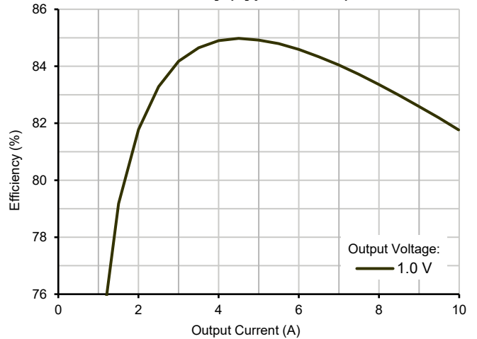
4.1.4 SVFA0510S Efficiency (Typical, 25 °C)
