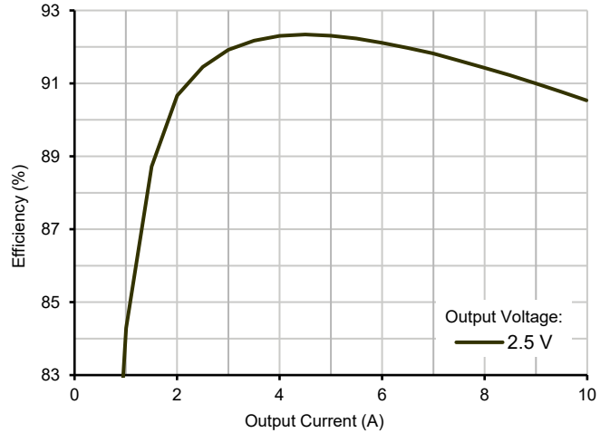
4.1.2 SVFA0510S Efficiency (Typical, 25 °C)
