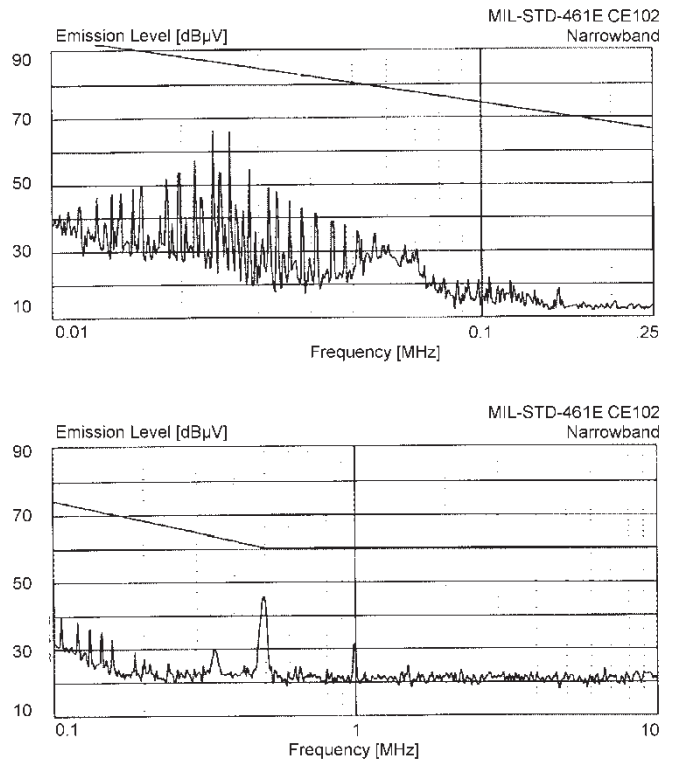
Figure 6 – MIL-STD-461D/E Two VPT5-2800S With VPTF1-28 EMI Filter
