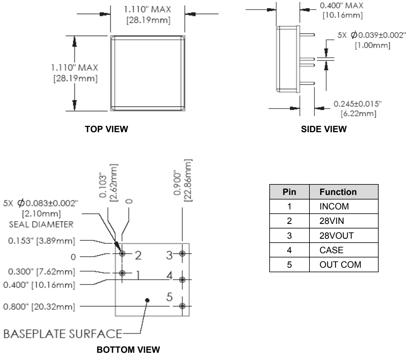
Figure 7 – Package and Pinout (Dimensional Limits are \pm 0.005 " Unless Otherwise Stated)
