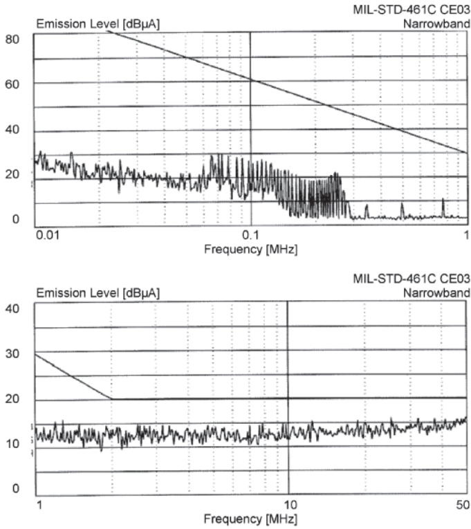
Figure 5 – MIL-STD-461C Two VPT5-2800S With VPTF1-28 EMI Filter
